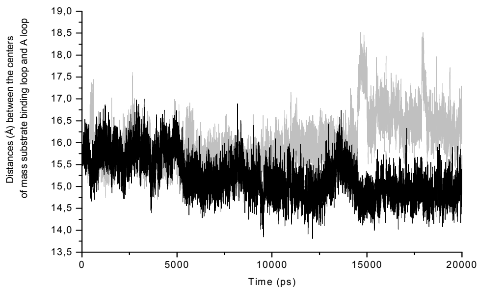
FIGURE 2 Distances (Å) between the centers of mass of the A-loop and the substrate binding loop at 298 K (gray) and 310 K (dark). \Delta D_{310-298} is 1,6 Å in the last 5.0 ns of the trajectory.
